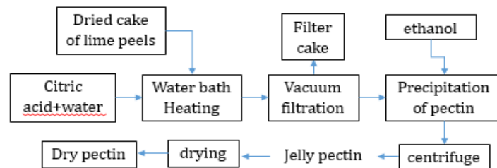
Figure 1. Process flow chart for extraction of pectin from lime peel residue
