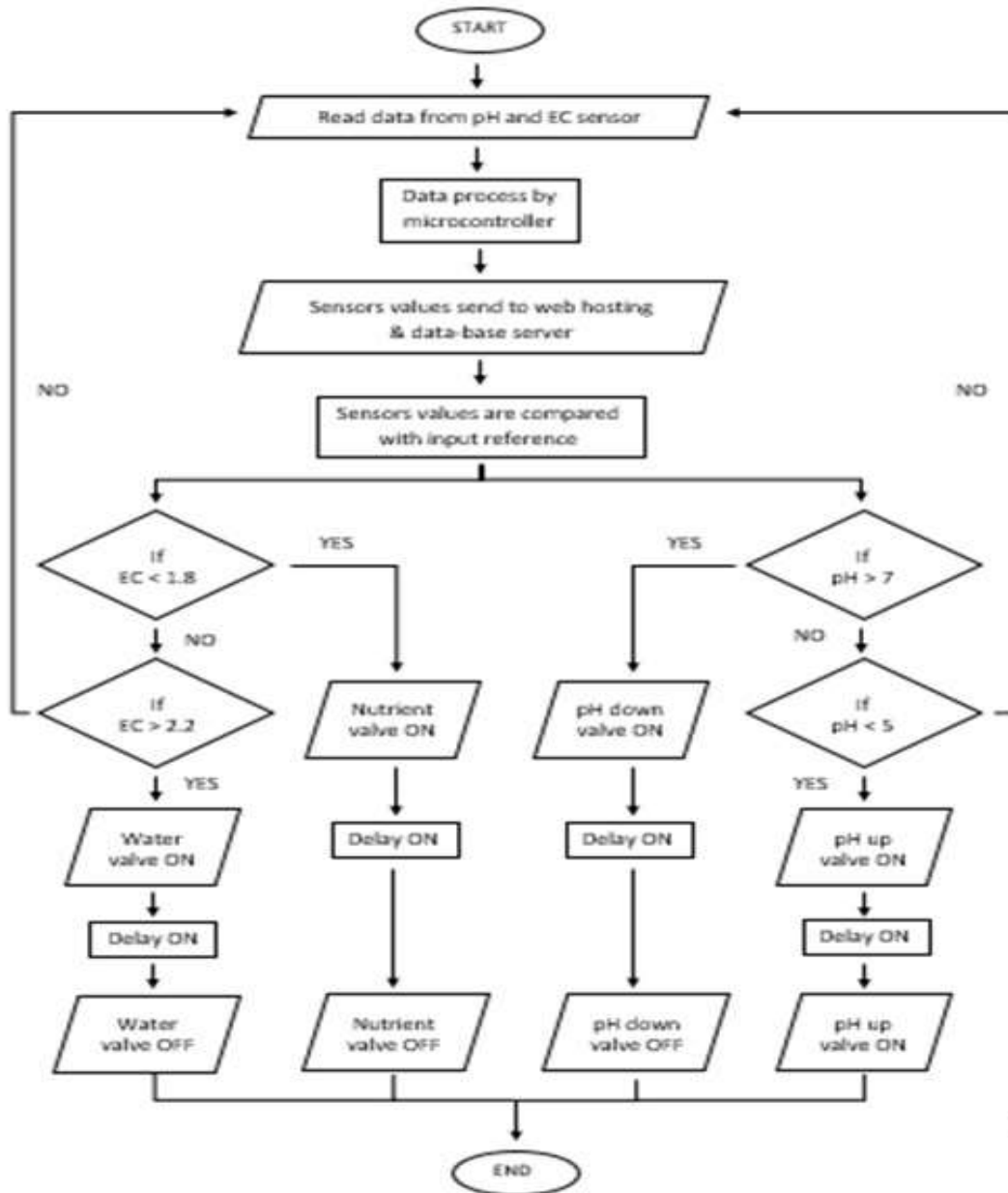
Figure 3. Flow chart of the overall system
