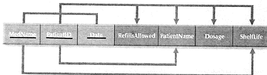
Figure 1: Unnormalized Relation
